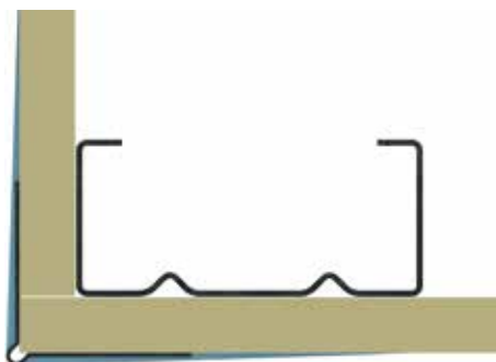
P32 External Corner Bead in situ
