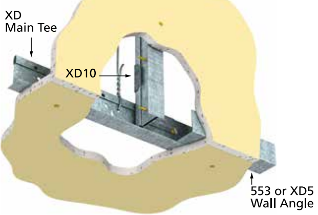
■ 90° OUTSIDE CORNER WITH MAIN TEE AT BOTTOM EDGE AND DETAIL
