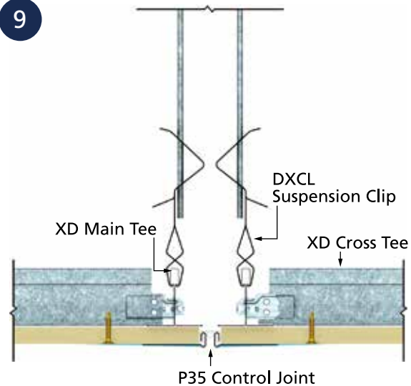
■ USING RONDO P35 CONTROL JOINT – NON FIRE-RATED
